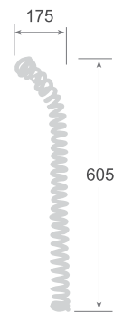
AISI 304 18/8 Muelle Inoxidable Stainless steel spring
